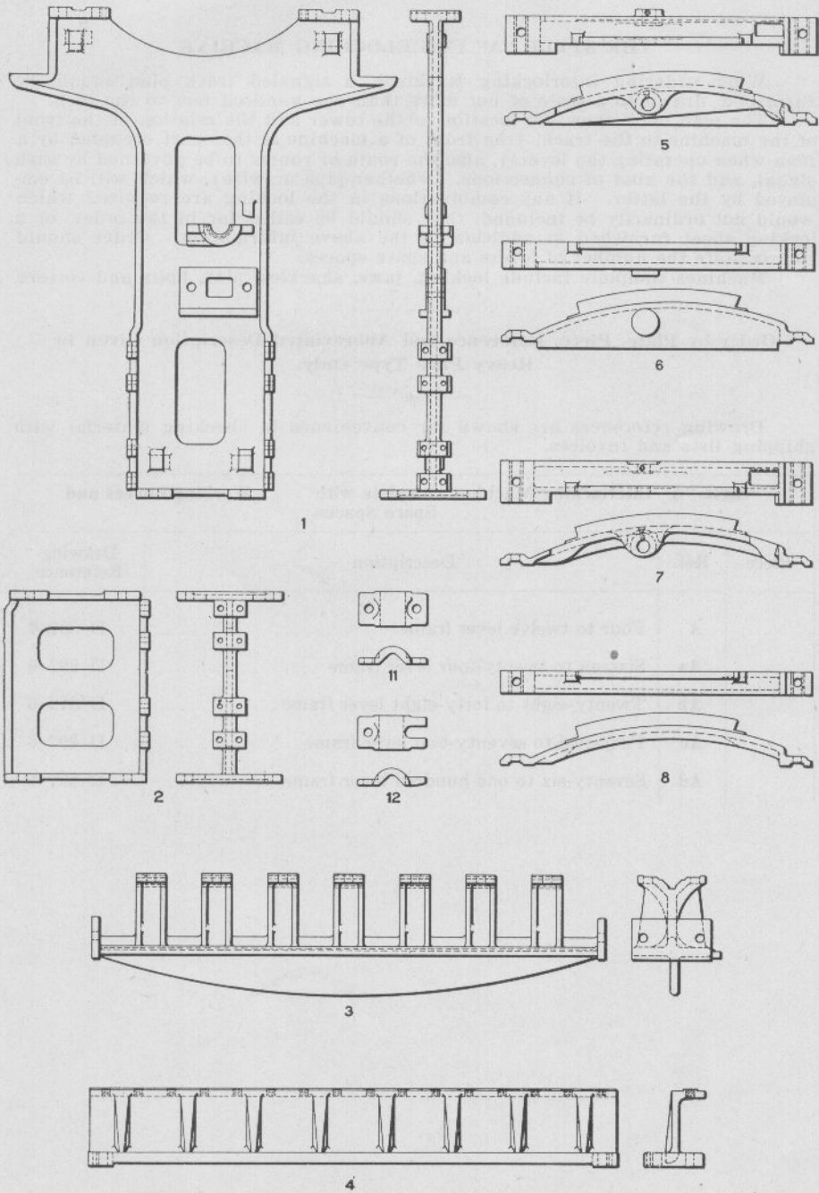
LEGS, GIRDERS, RAILS, QUADRANTS, ETC., FOR STYLE "A" INTERLOCKING MACHINE
